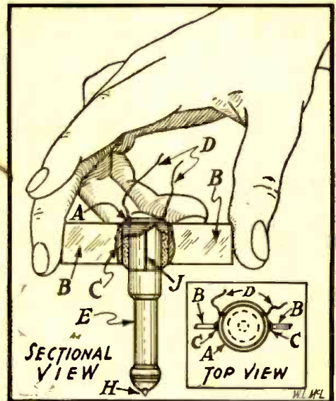
Fig. 1—Stylus assembly. Coding given below.
