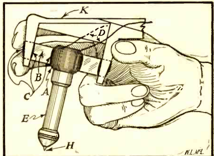
Photo, left—Exploded view of pickup. Fig. 2, below—Stylus in its frame. A—Coil. B—Plastic vane. C—Cement seal. D—Leads. E—Duraluminum stylus. H—Diamond tip. J—Split sleeve. K—Plastic frame.
