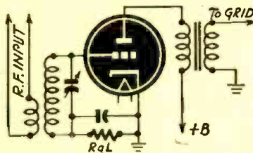
Fig. 3—Grid-leak is like a diode detector.
