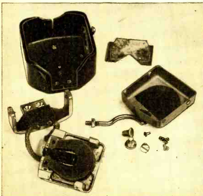
Photo, left—Exploded view of pickup. Fig. 2, below—Stylus in its frame. A—Coil. B—Plastic vane. C—Cement seal. D—Leads. E—Duraluminum stylus. H—Diamond tip. J—Split sleeve. K—Plastic frame.
