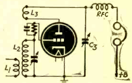
Fig. 5—Typical grid-leak-condenser circuit.
