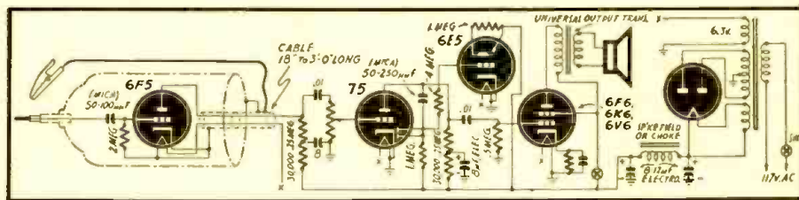
The complete Signal Tracer. A switch is provided so either 6E5 or speaker can be used.
