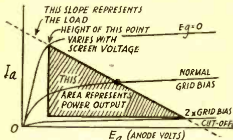
Fig. 1—Effect of screen feedback on power.
